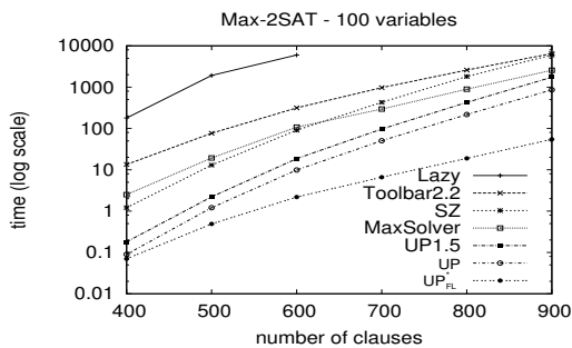
Figure 3: Comparison of Max-SAT solvers on Max-2SAT
