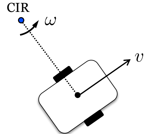
Robot unicycle
