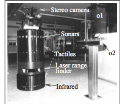
Fig. 3: The Robot and its sensors.
