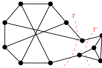
Fig. 8. A nonplanar nonbipartite cubic graph with two nontrivial tight cuts T and T' , which is 3-edge-colorable by Corollary 25.
