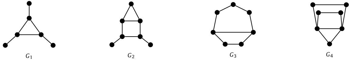
Fig. 3. The graphs G_i , i = 1, 2, 3, 4 , are the subgraphs that prevent the matching polytope from being box-TDI (up to fully odd subdivision).
