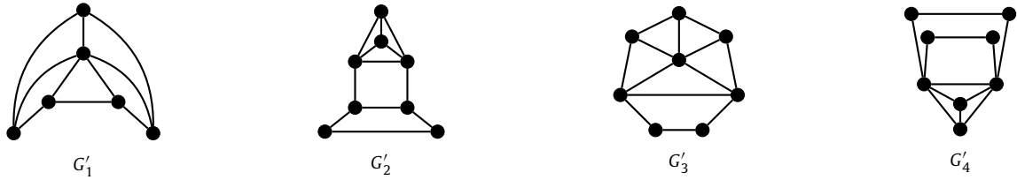
Fig. 4. The graphs G'_1 , G'_2 , G'_3 , and G'_4 are matching covered graphs whose perfect matching polytope is box-TDI, yet their matching polytope is not.
