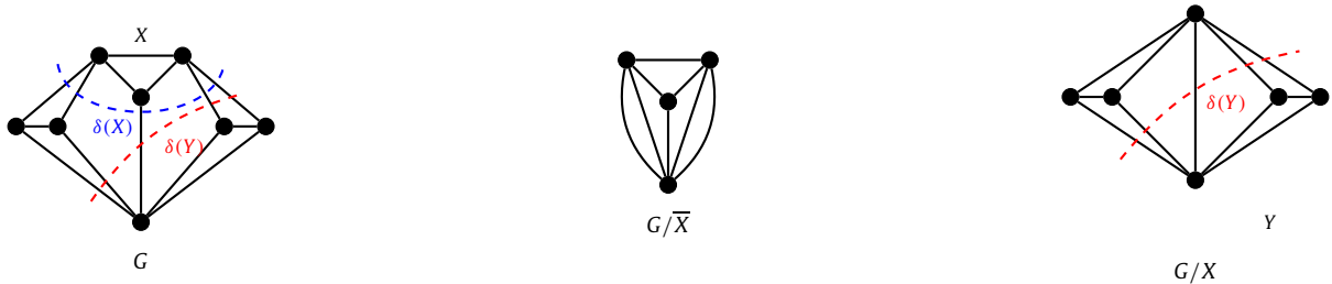
Fig. 2. A matching covered graph G , and a maximal inclusionwise laminar family of tight cuts \mathcal{F} = \{\delta(X), \delta(Y)\} . As \mathcal{F} \in \mathfrak{F}_G , G has three bricks. In particular, one can see the two \delta(X) -contractions G/X and G/\bar{X} . While G/\bar{X} is already one of the bricks of G , G/X still has two bricks that one can identify by computing G/X/Y and G/X/\bar{Y} . All of these bricks are isomorphic to K_4 , up to parallel edges.
