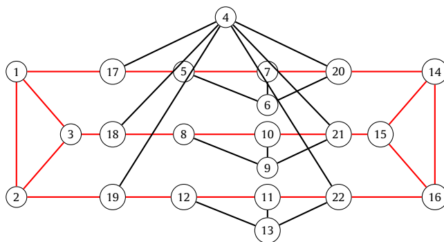
Fig. 7. A matching covered graph containing a fully odd subdivision of \overline{C}_6 (in red) as a subgraph and whose perfect matching polytope is box-TDI.
