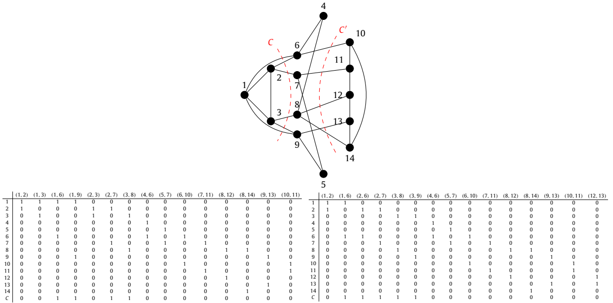
Fig. 6. The Moonfish graph \mathcal{M} and the unique maximal inclusionwise laminar family \{C, C'\} of \mathcal{M} . One can check that all C -contractions and C' -contractions are odd intercylic near-bricks. Since, \mathcal{M} has two bricks -K_4 and the odd wheel of order 5— and the two C -contractions are nonbipartite, \{C\} \in \mathfrak{F}_{\mathcal{M}} . In particular, the two matrices above are nonsingular maximal submatrices of on the M_{\mathcal{M}}^{(C)} and have —from left to right— determinant 4 and 8, up to the sign. Then, the matrix M_{\mathcal{M}}^{(C)} is nonequimodular, by definition, and it is face-defining for the affine hull of P(\mathcal{M}) by Theorem 9. By Theorem 11, P(\mathcal{M}) is not box-TDI.
