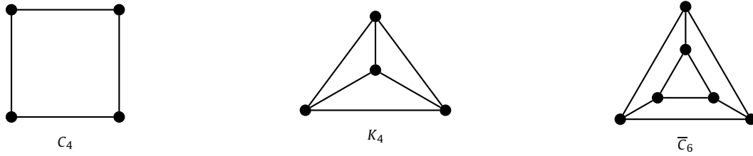
Fig. 1. From left to right: the brace C_4 , which is the smallest solid bipartite graph; the brick K_4 , which is the smallest solid nonbipartite graph; the brick \bar{C}_6 , which is the smallest nonsolid brick.
