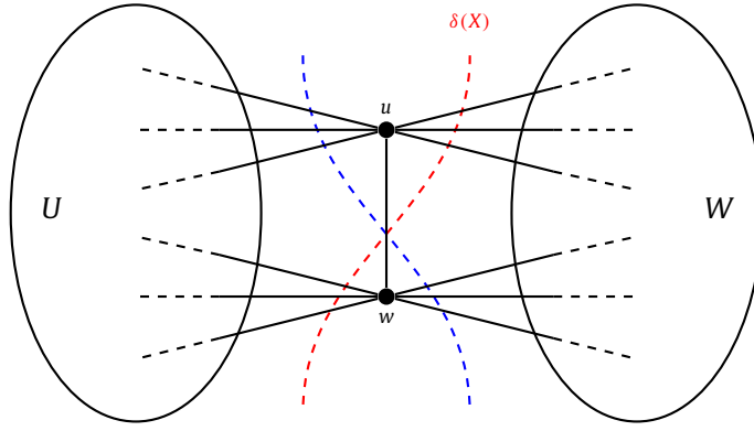
Fig. 5. The two 2-separation cuts with respect to u and w are drawn in red and blue. Note that u and w may be nonadjacent.
